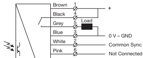
SGR 16 Load as PNP output
