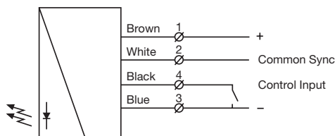
SGT 16 Control wire for test input and static blanking function (blanking function in C1 models only)
