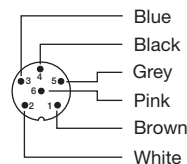
6 pin, M8 Cable Plug (Female)
