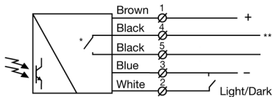
* Relay type: Open when SGR is not powered ** Max. 24 V ac / 36 V dc
