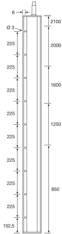
SGR Rear View
