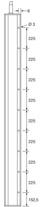
SGT Rear View
